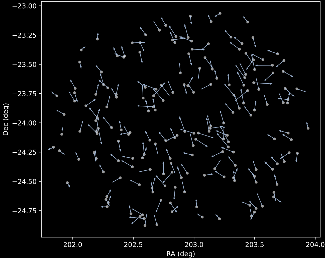
GALAH DR4 Cluster 1 Proper Motion Vectors (n=189)
