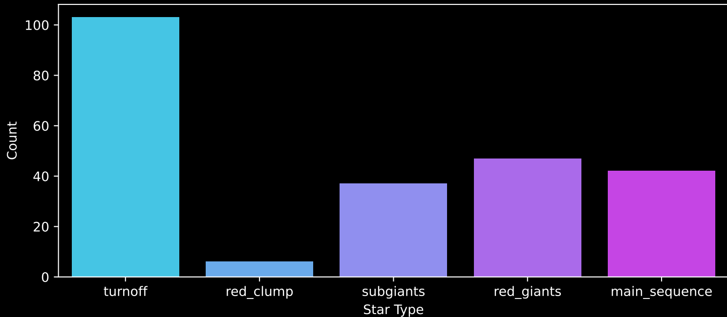
GALAH DR4 Field: [8435] Count plot of Star Type
