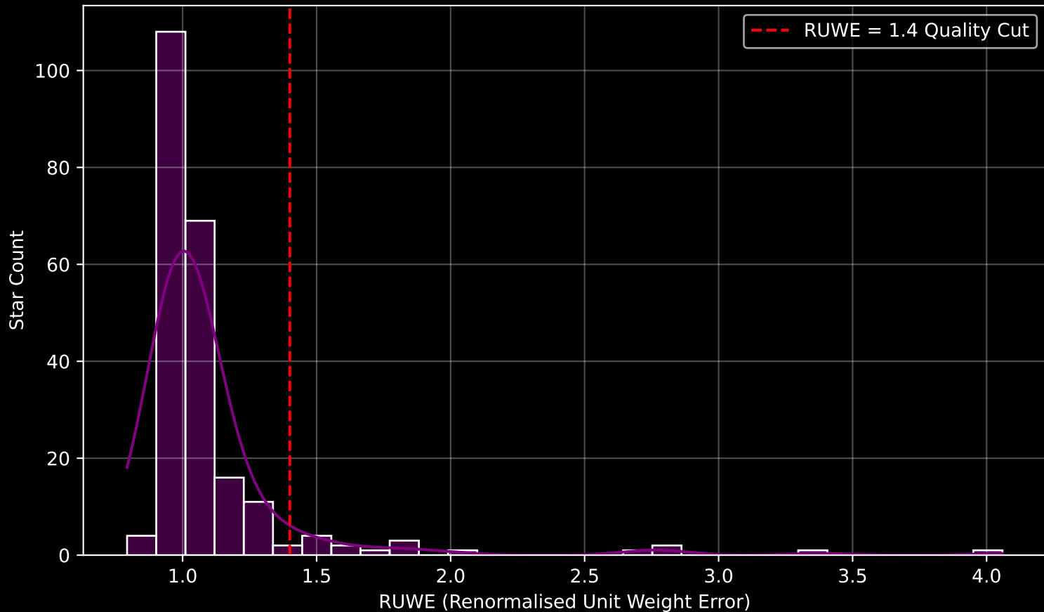
GALAH DR4 Field [8435] RUWE Distribution (n= 226)
